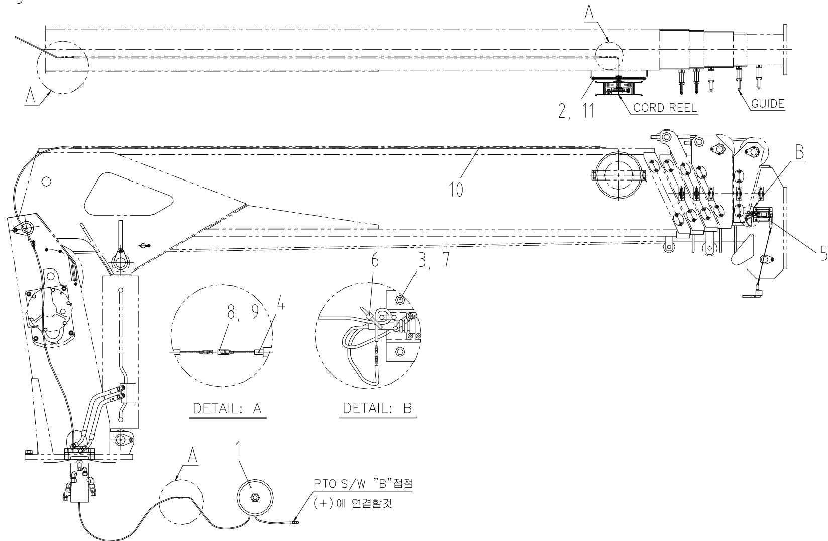
Fig. 9 SCS736 OVERWINDING ALARM DEVICE ASS'Y
