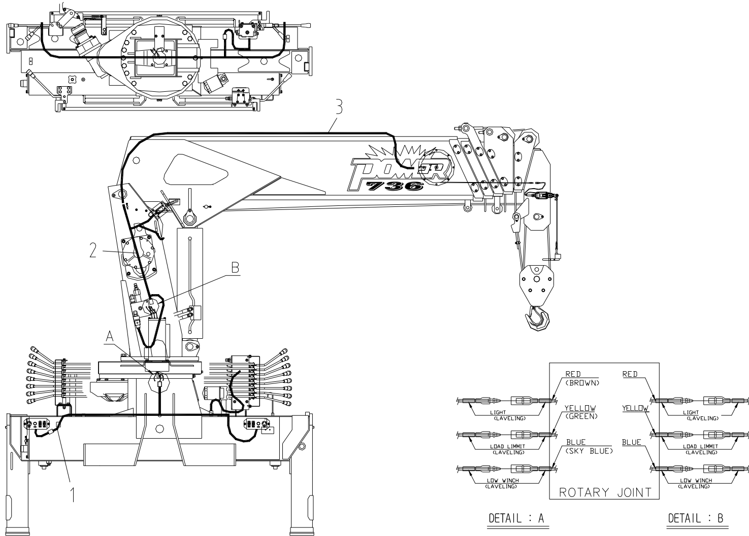
Fig. 11 SCS736 WIRING ASS'Y
